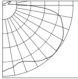
BIS175MXX-CLO-GEP TEST NUMBER: 26240 LAMP: 175W MH, COATED LUMENS: 15,000 MOUNTING HEIGHT: 12 FEET
