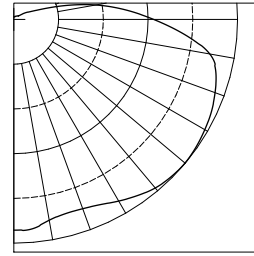
BIS42CCXX-CLO-GEP TEST NUMBER: 26291 LAMP: 42W CFL LUMENS: 3,200 MOUNTING HEIGHT: 12 FEET
