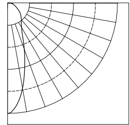
BIS18WLXX-CLO-GE TEST NUMBER: 27584 LAMP: 18W LED NEUTRAL WHITE LUMENS: 700 MOUNTING HEIGHT: 12 FEET
